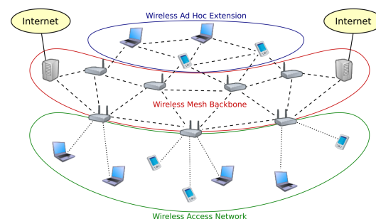
Figure 1. MobiMESH Network Architecture
