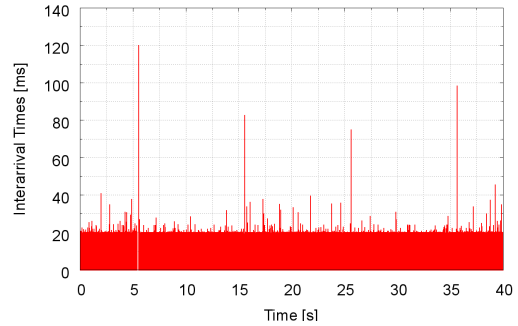
Figure 2. Mobility delay on a VoIP call
